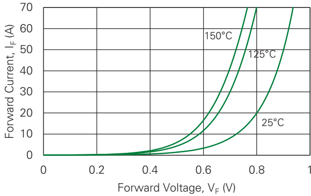
Figure 1. Maximum Forward Voltage Drop Characteristics
