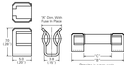
111 505 Device Dimensions
