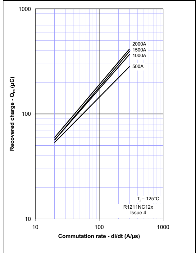
Figure 6 - Recovered charge, Q_{ra} (50% chord) ( \mu\text{C} )
