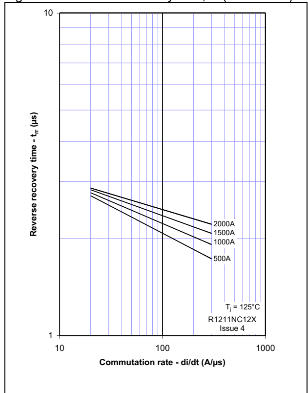
Figure 8 - Maximum recovery time, t_{rr} (50% chord) ( \mu\text{s} )
