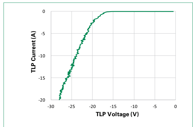
AQHV12-C Negative Transmission Line Pulsing(TLP) Plot
