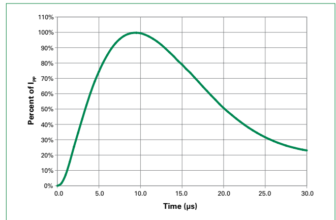
8/20 \mu\text{s} Pulse Waveform
