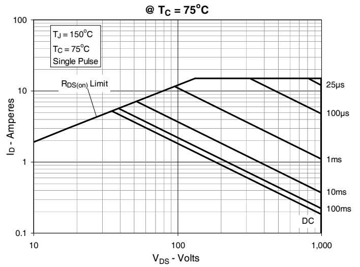
Fig. 16. Forward-Bias Safe Operating Area @ T_C = 75^\circ C
