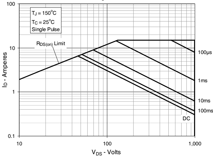
Fig. 15. Forward-Bias Safe Operating Area @ T_C = 25^\circ C
