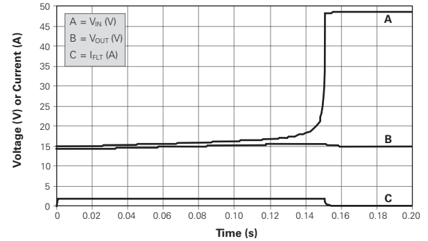
Figure PZ34 Typical Fault Response: ZEN132V075A48LS 48V, 2.0A Current Limited Source ( I_{OUT}=0 )
