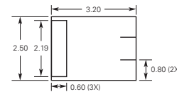
Recommended Pad Dimensions (mm)
