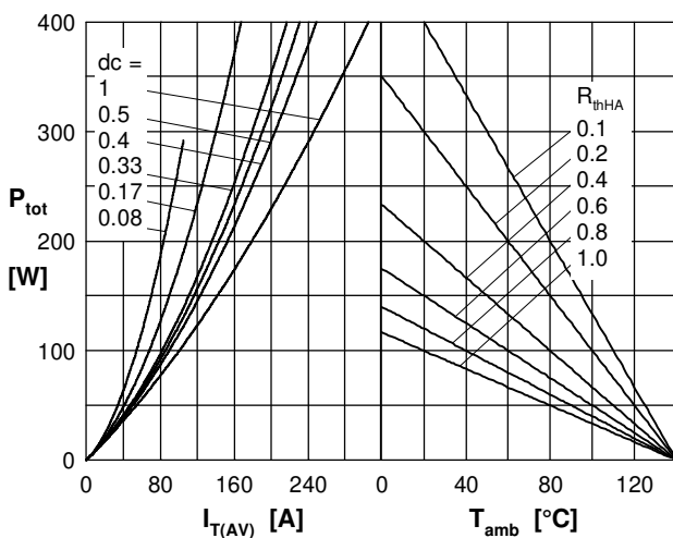
Fig. 7a Power dissipation versus direct output current
