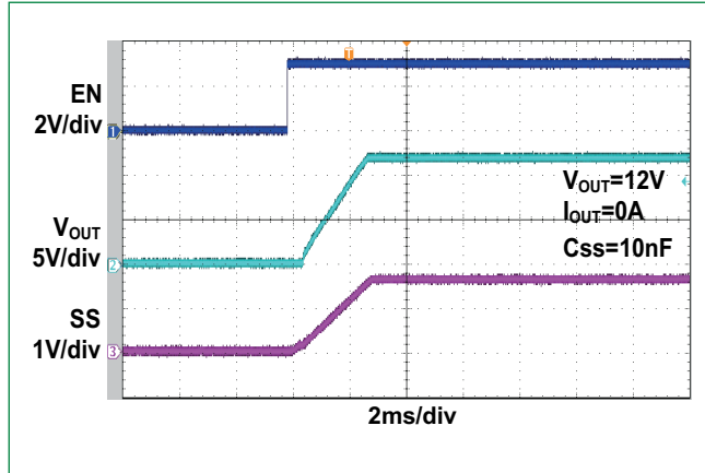
Soft Start Time
