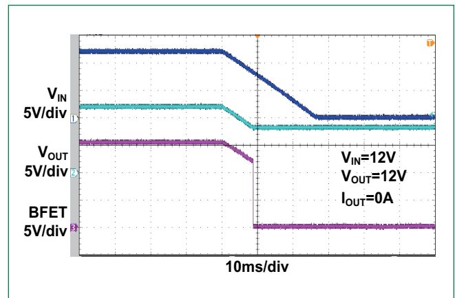
Turnoff Delay to BFET
