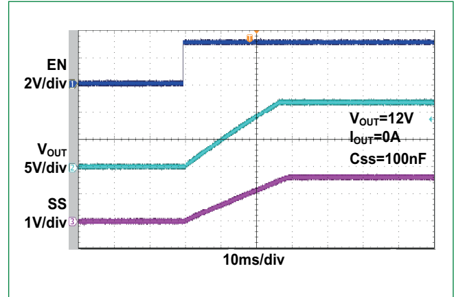
Soft Start Time
