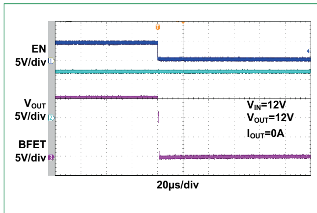
Turnoff Delay to BFET
