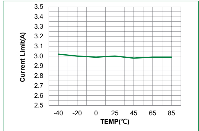
Programmable Current Limit (RLIM=3.3K)
