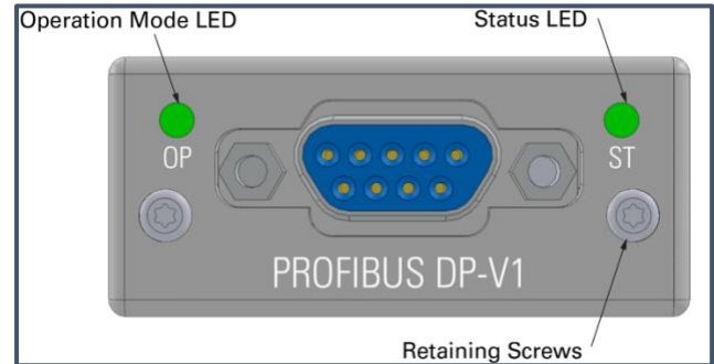
FIGURE 1. LED Indicators.
