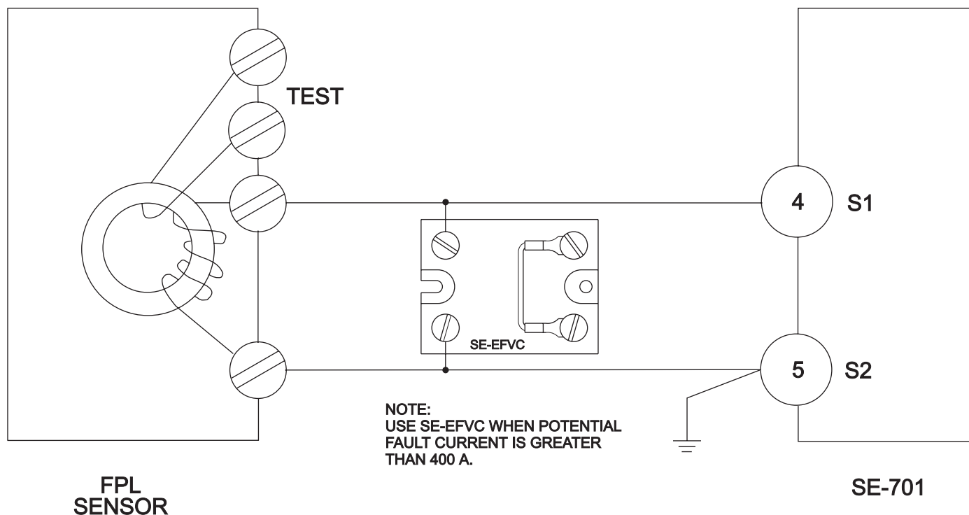
FIGURE 1. Connection Diagram for SE-701.
