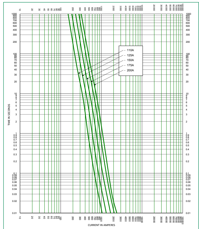
Time Current Curve JLLS (110–200 A)
