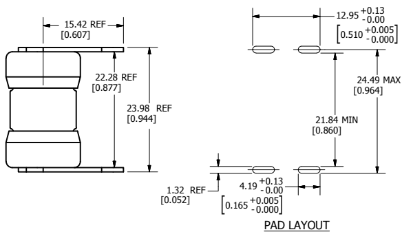
PAD LAYOUT
