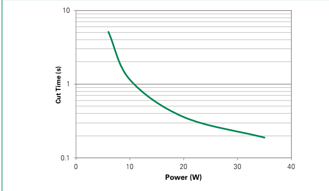
Various heater wattage at 25°C ambient temperature
