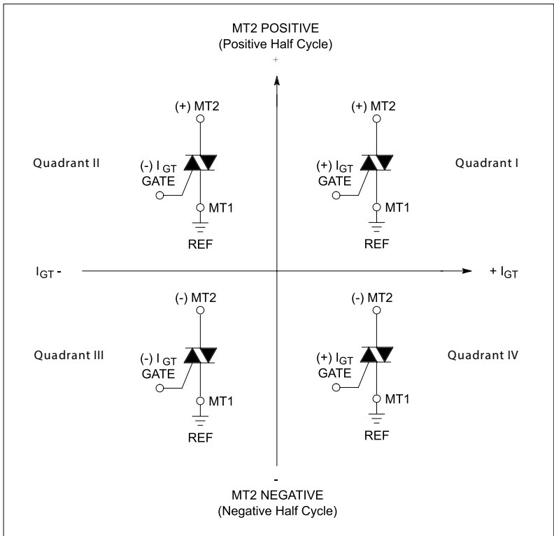
All polarities are referenced to MT1. With in-phase signals (using standard AC lines) quadrants I and III are used.
