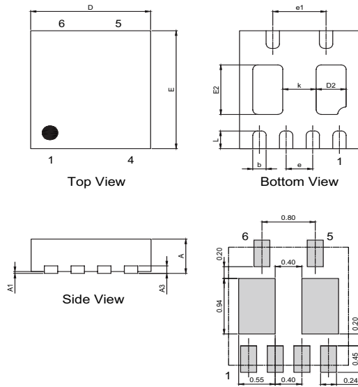
Recommended soldering pad layout (Unit : mm)
