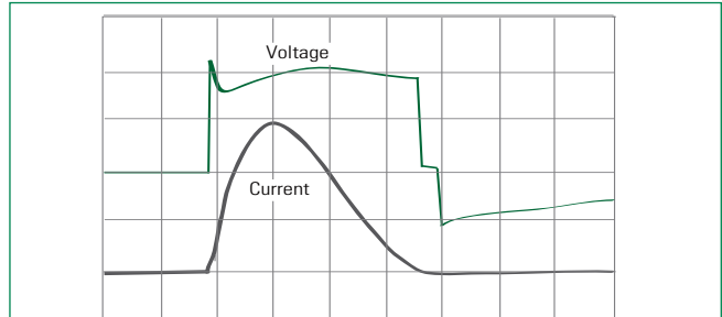
Figure 6 -Surge Response (8/20 Surge current waveform)
