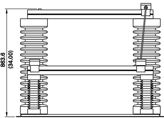
RIGHT SIDE
