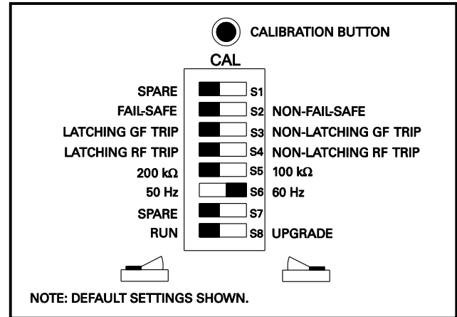
FIGURE 1. Configuration Switches.
