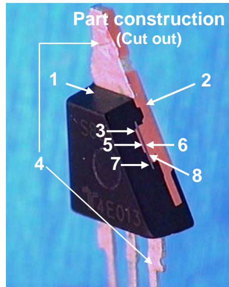
TO-220 R Package (shown) TO-263 N Package (Non-isolated)
