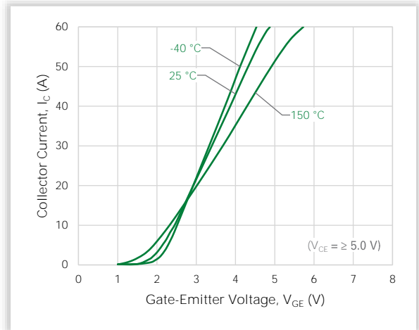
Figure 8. Transfer Characteristics
